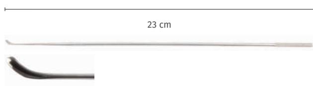
Messer, golfstockförmig, AL 23 cm Knife, golf club shaped, WL 23 cm
