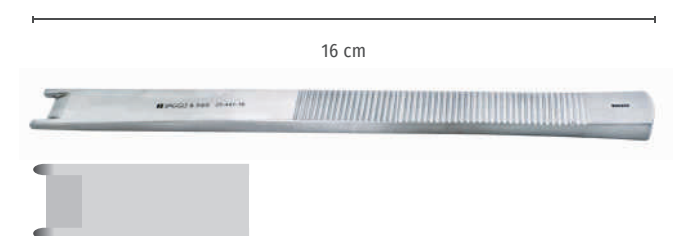
Masing Osteotom, 2 Führungsdorne, 10 mm-Schneide, gerade, 16 cm Masing osteotome, 2 guards, 10 mm blade, straight, 16 cm
